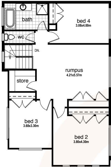
UPPER FLOOR LAYOUT
